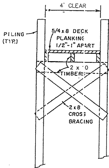
BOARDWALK DETAIL NOT TO SCALE
